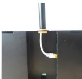
Step 3 Plug the cable
